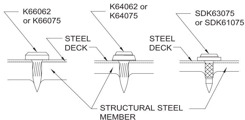
FIGURE 8 – PNEUTEK FASTENERS
