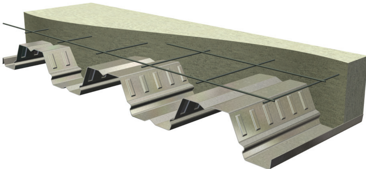
PLW3™ FORMLOK™ and W3 FORMLOK™
