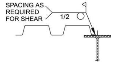
1 PARALLEL SUPPORTS
