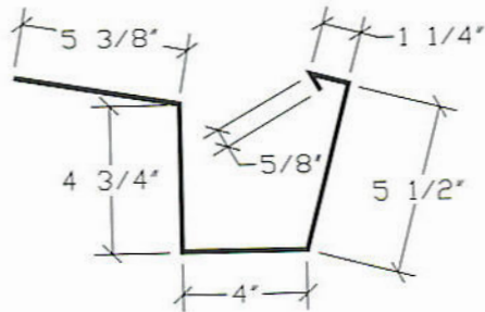
Box Gutter (GU6) pre-hung
