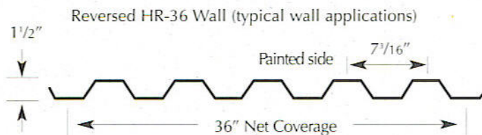
Reversed HR-36 Wall Section Properties
