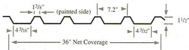
Reversed Box Rib (Recommended for roof application)
