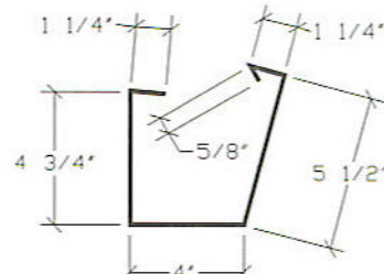
Box Gutter (GU8) post-hung
