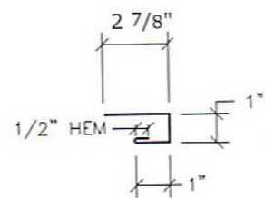
C-Metal (C-13) Nu-Wave & U-Panel
