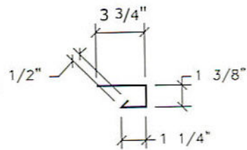
Jamb Trim (J6) Super Span only
