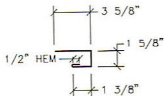
C-Metal (C11) Box Rib & HR-36
