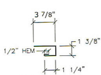
C-Metal (C-6) Super Span only
